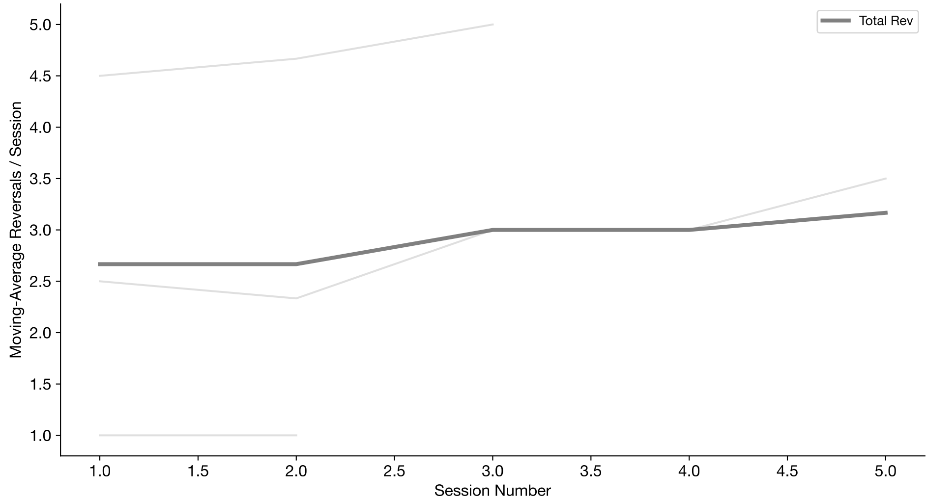
Moving-Average Total Reversals Over Time (n=3 subjects; sessions per subject=2-5; window=3)
